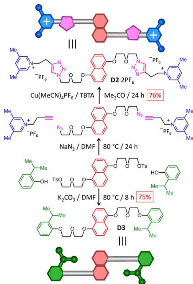
Scheme 2. Synthesis of Dumbbells D2 \cdot 2PF_6 and D3 and Their Graphical Representations
