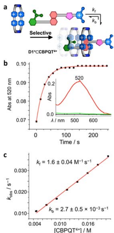
Figure 3. UV/vis absorption spectroscopy determination of the kinetic barrier to threading the 2-isopropylphenyl terminus through \text{CBPQT}^{4+} . (a) Graphical representation of the selective threading leading to the formation of inclusion complex \text{D1}^+\text{CCBPQT}^{4+} . (b) Kinetic trace for the formation of \text{D1}^+\text{CCBPQT}^{4+} obtained by tracking the absorbance at 520 nm in the UV/vis absorption spectra recorded in MeCN at 298 K. The spectra were recorded every 14.5 s in a 1 mm cell-path-length cuvette. A single rate-limiting step is observed. [\text{D1}^+]_0 = 1.5 \times 10^{-3} \text{ M} ; [\text{CBPQT}^{4+}]_0 = 2.0 \times 10^{-2} \text{ M} . (Inset) UV/vis absorption spectra of \text{CBPQT}^{4+} (black trace), \text{D1}^+ (green trace), and \text{D1}^+\text{CCBPQT}^{4+} (red trace) recorded in MeCN at 298 K. The formation of \text{D1}^+\text{CCBPQT}^{4+} is characterized by a charge-transfer band centered close to 520 nm. (c) Plot of the apparent pseudo-first-order rate constant, k_{\text{obs}} , vs the concentration of \text{CBPQT}^{4+} , with the concentration of \text{D1}^+ held constant (i.e., [\text{D1}^+]_0 = 1.5 \times 10^{-3} \text{ M} ). Solvent, MeCN; T = 298 \text{ K} .
